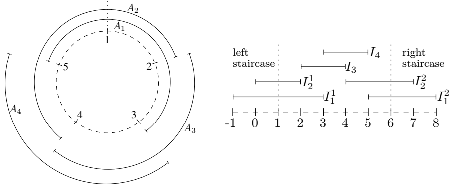
Figure 2: Instance of ARCCOLORING (left), constructed intervals (right)
