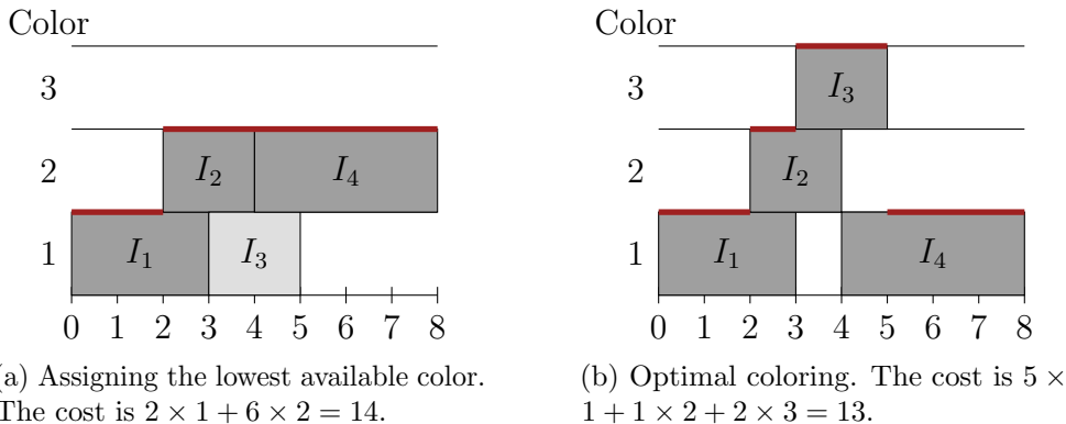
Figure 1: Two different colorings of four intervals. An optimal solution does not necessarily minimize the number of colors used. The darker intervals contribute to the cost of the coloring but the lighter interval does not. The bolded line indicates the skyline.
