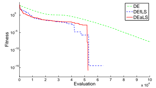
Figure 6: Convergence curve for f_{grw} function.
