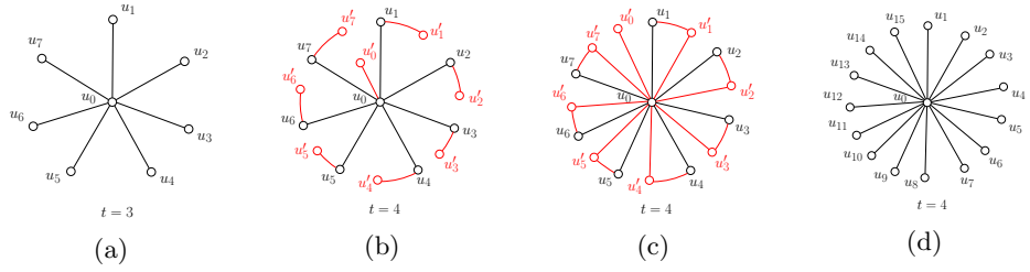
Fig. 1: The operations of the star graph process in slot t = 4 . (a) A star of size 2^3 grown by the end of slot 3. (b) For every u_i , a vertex u'_i is generated by the process and is connected to u_i . (c) New vertices u'_i are connected to u_0 . (d) Edges between peripheral-vertices are being removed to obtain the star of size 2^4 grown by the end of slot 4. Here, we also rename the vertices for clarity.
