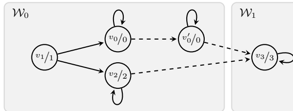
Fig. 7. A tradeoff between resilience and semantic quality (measured in the maximal color occurring infinitely often).
