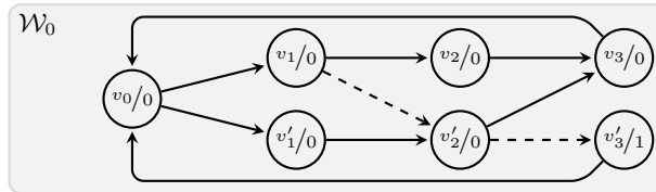
Fig. 5. Moving from v_0 to v_1 allows Player 0 to minimize visits to odd colors, while moving to v'_1 allows her to minimize the occurrence of disturbances.
