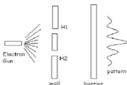
Electrons
