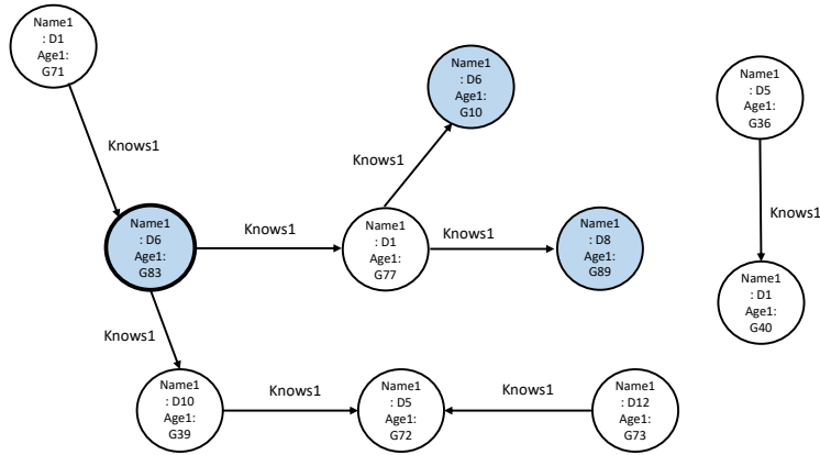
Figure 4: Traversal-aware encryption adjustment. Ciphertexts shown are not full-length.
