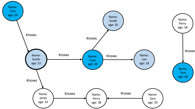
Figure 1: Data layout at the server of the graph database.
