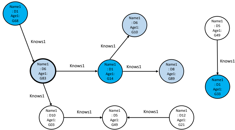
Figure 3: The encryption is adjusted to DET layer.
