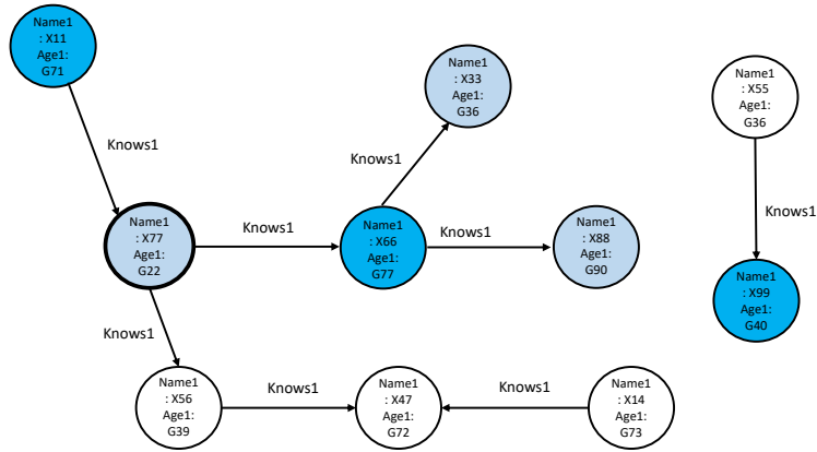
Figure 2: The nodes created at the DBMS server. The encryption is set at RND layer everywhere. Ciphertexts shown are not full-length.
